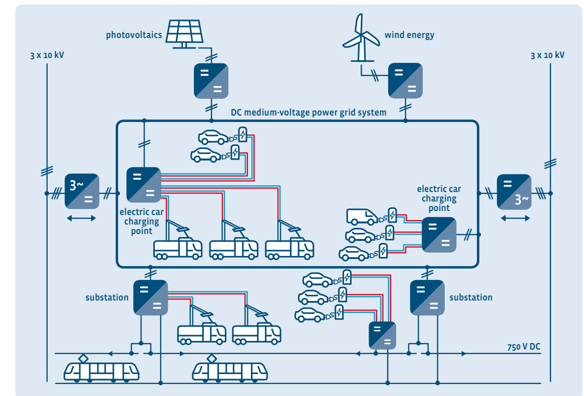
Figure 6: Connecting e-vehicle charging stations to the existing public transport infrastructure
