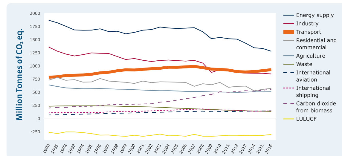
Figure 2: Development of emissions by sector in Europe since 1990 2
