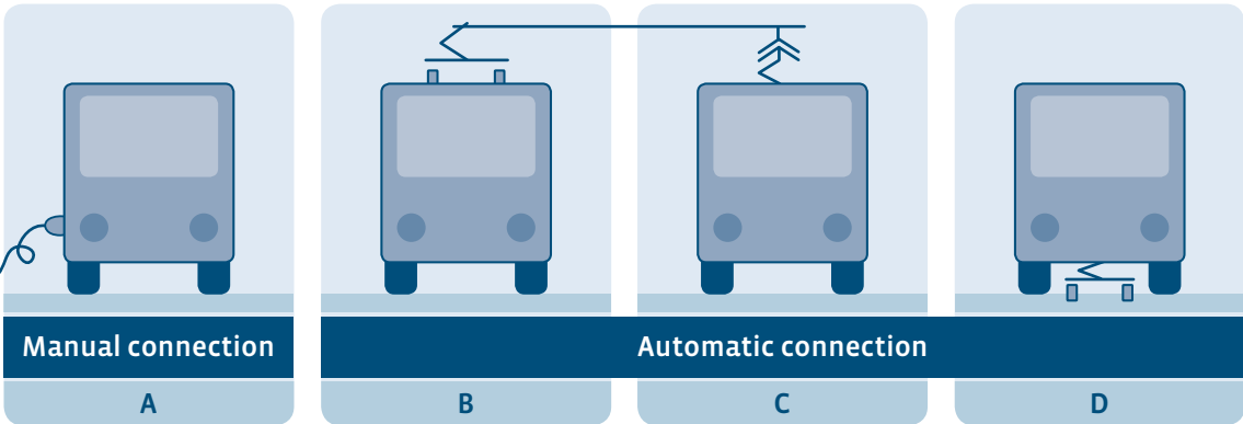
Figure 5: Overview of different technical charging solutions A (plug in), B (pantograph going down), C (pantograph going up) and D (pantograph below vehicle), (Source UITP, April 2018)
